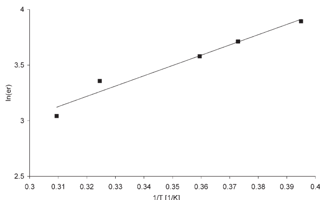
Figure 5. Eyring plot [ \ln(e_r) vs. 1/T ]. Temperature dependence of the enantiomeric excess achieved by ligand ( S_p,S )- 3 . 1) C_6H_{11}CHO (0.5 mmol), 2 mol % of ligand, 1 mL of Et_2Zn (1 M in hexanes), 1 mL of toluene, 12 h; 2) Ac_2O , 24 h, room temperature.
