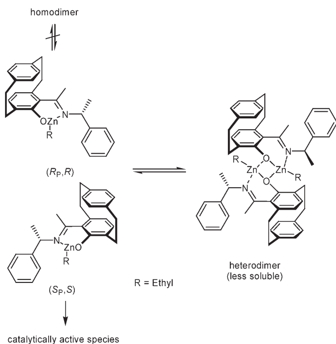
Scheme 1. Equilibria of ligands 1 .
