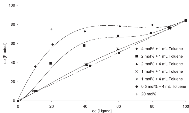
Figure 2. Results for the studies of the non-linear effect of the ligands ( S p S )/( R p R )-1. 1) C_6H_{11}CHO (0.5 mmol), 0.5–4 mol % of ligand, 1 mL of Et_2Zn (1 M in hexanes), 1–4 mL of toluene, 0 °C, 12 h; 2) Ac_2O , 24 h, room temperature.
