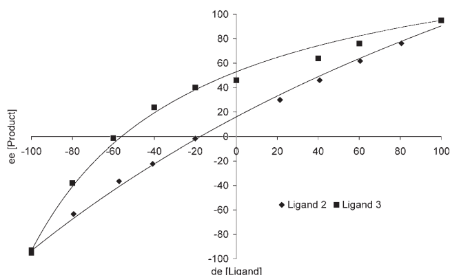
Figure 4. Activity studies with different ratios between the diastereomeric pair ( S )- 2 and ( S )- 3 , respectively. 1) C_6H_{11}CHO (0.5 mmol), 2 mol % of ligand, 1 mL of Et_2Zn (1 M in hexanes), 1 mL of toluene, 0 °C, 12 h; 2) Ac_2O , 24 h, room temperature.
