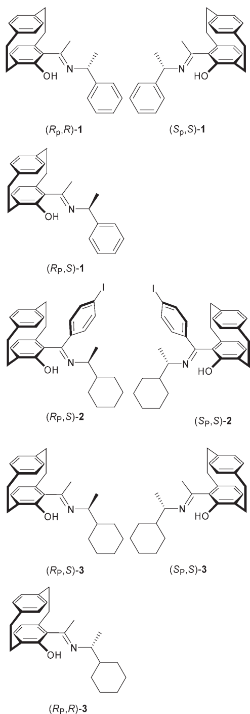
Figure 1. Planar- and central-chiral N,O -[2.2]paracyclophane ligands.
