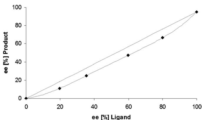
Figure 3. Results for the non-linear effect studies for the ligands (S_p,S)/(R_p,R) - 3 . 1) \text{C}_6\text{H}_{11}\text{CHO} (0.5 mmol), 4 mol % of ligand, 1 mL of \text{Et}_2\text{Zn} (1 M in hexanes), 1 mL of toluene, 0^\circ\text{C} , 12 h; 2) \text{Ac}_2\text{O} , 24 h, room temperature.
